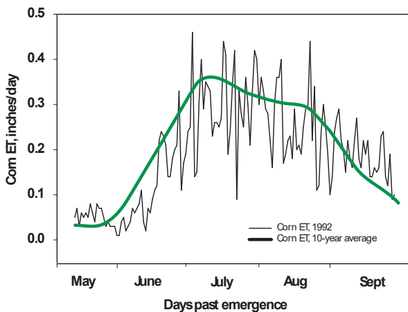
Figure 26. Daily vs. 10-year average ET in Burlington, CO.
