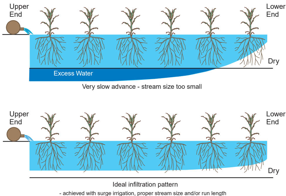
Figure 32. Surface irrigation infiltration patterns.
